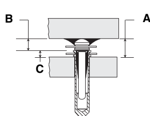
Figure 2 Surface Mount
